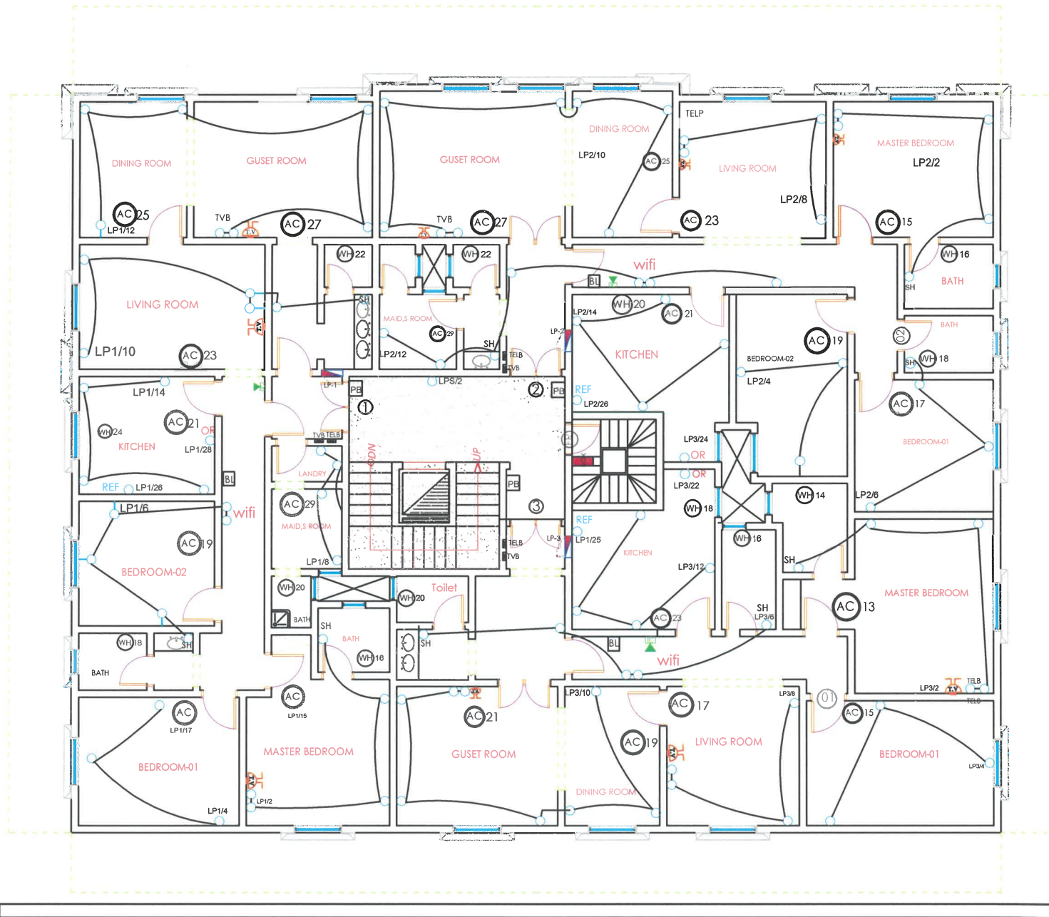
TYPICAL FLOOR POWER&TEL&TV PLAN SCALE: 1:200 MTS.
